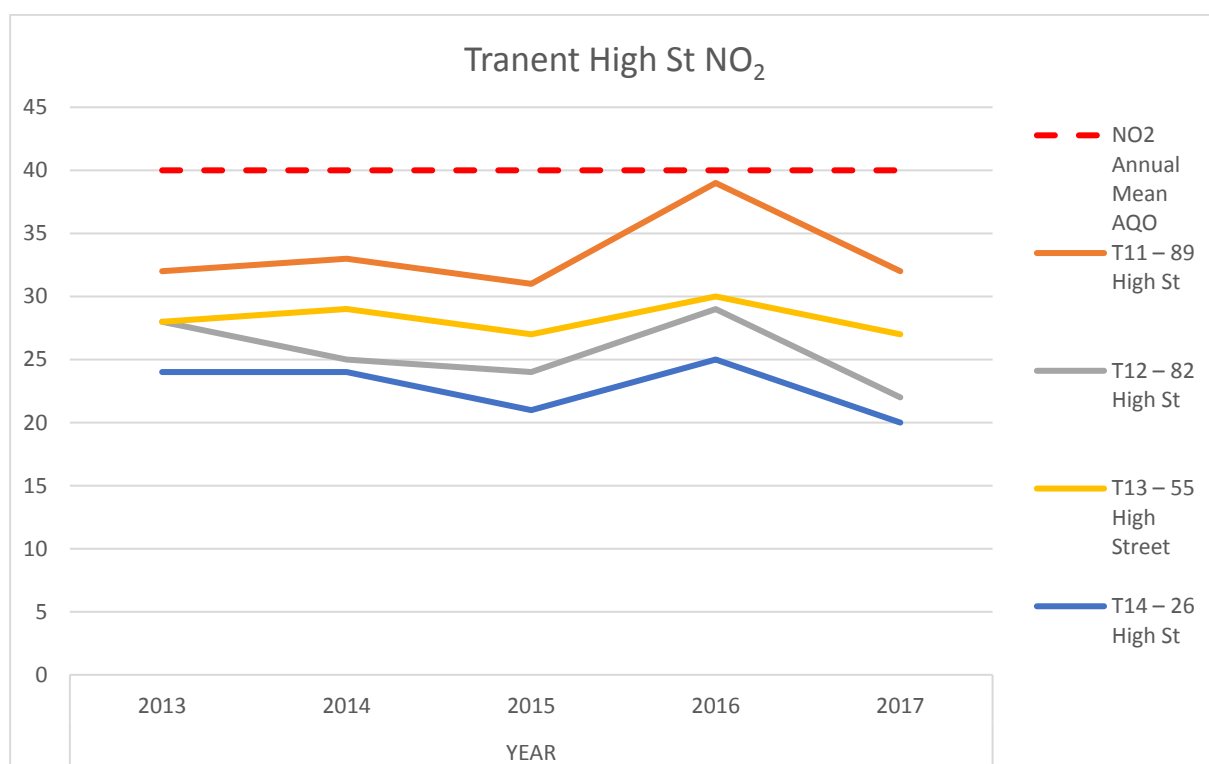
Figure 2: Diffusion Tubes on Tranent High Street 2013-2017
