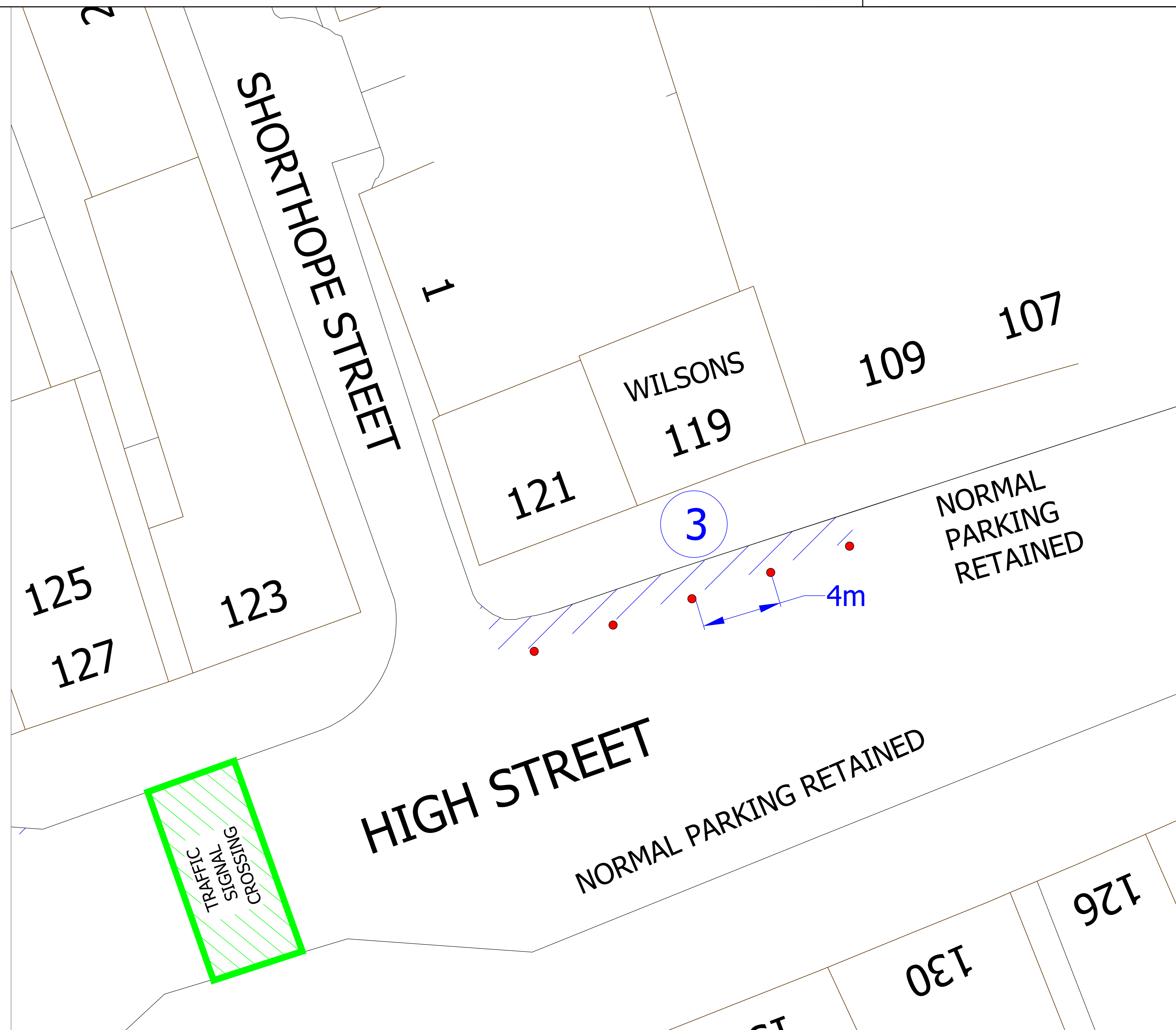
MUSSELBURGH HIGH STREET - STAGE 1 - SECTION 3 1:100 (A0)
