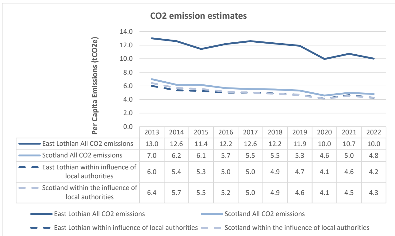
Figure 43: CO2 Emission estimates per capita (tonnes per capita) in East Lothian and Scotland (UK Government 2016)
