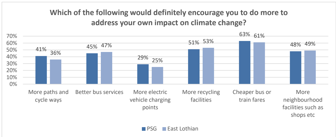
Figure 42:- Impact on climate change (East Lothian Council Residents Survey 2024)
